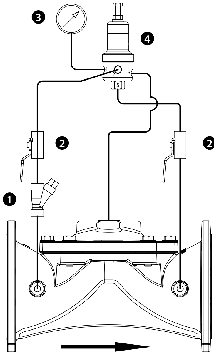
Pressure Sustaining Control Valve - 2 Way
